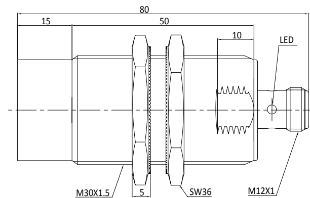
Fig. 4 Inductive sensor with M12 connector (non-flush)
