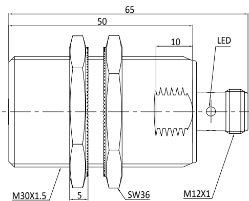
Fig. 3 Inductive sensor with M12 connector (flush)
